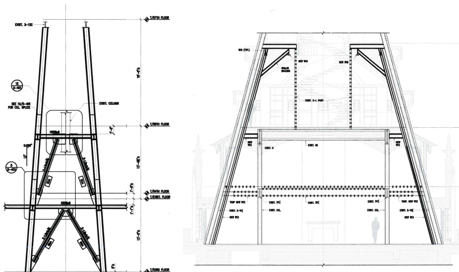
Figure 8. Pinnacle reinforcement.
